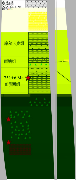
Fig.4 Stratigraphic
